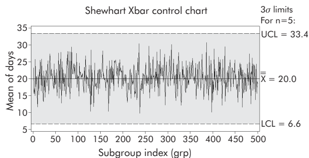
Figure 3 Structure of an Xbar (mean) control chart. The center line indicates the grand mean of the process when in control. The upper (UCL) and the lower (LCL) dashed lines represent the upper and lower control limits calculated as 3-sigma. Points in the graph correspond to average for blocks of size five observations each. All points are contained within the 3-sigma limit.
